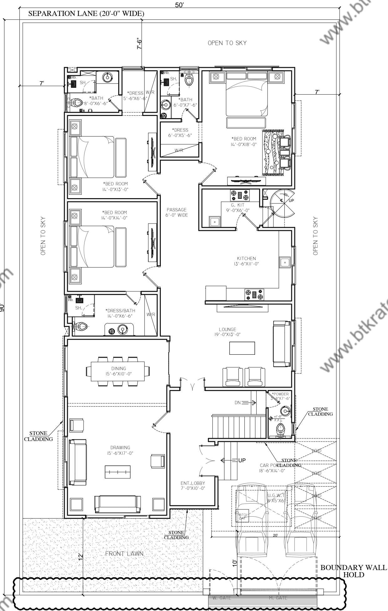
GROUND FLOOR PLAN COVERED AREA = 2524.25 SQ.FTS ROAD 15-A (80'-0" WIDE)
