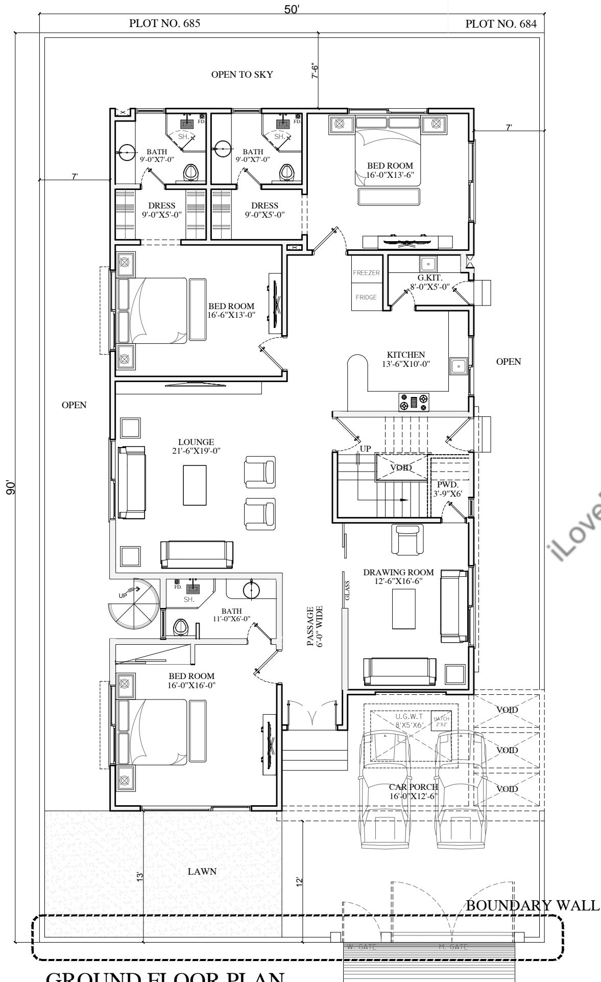
GROUND FLOOR PLAN COVERED AREA = 2472.00 SQ,FTS
