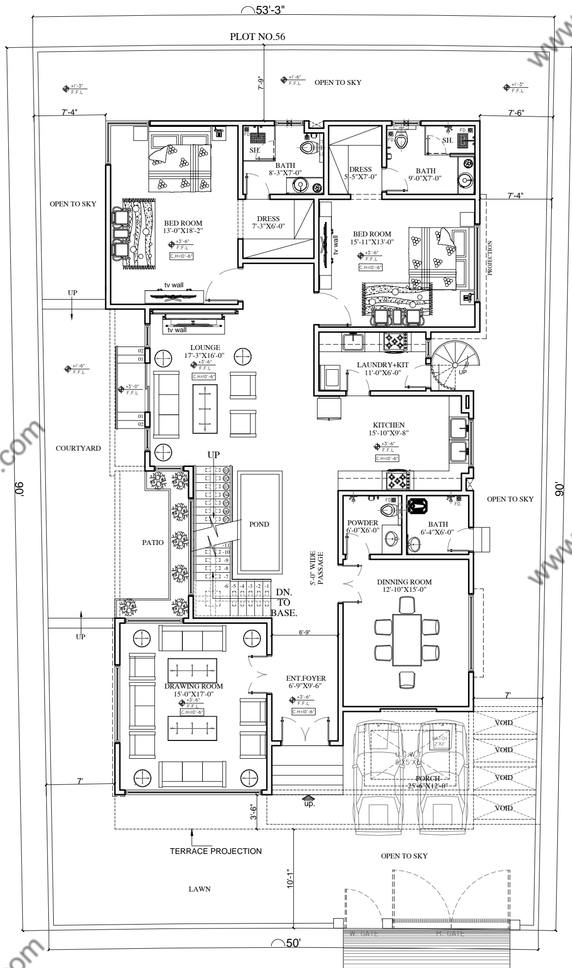
GROUND FLOOR PLAN COVERED AREA = 2648.59 SQ.FTS
