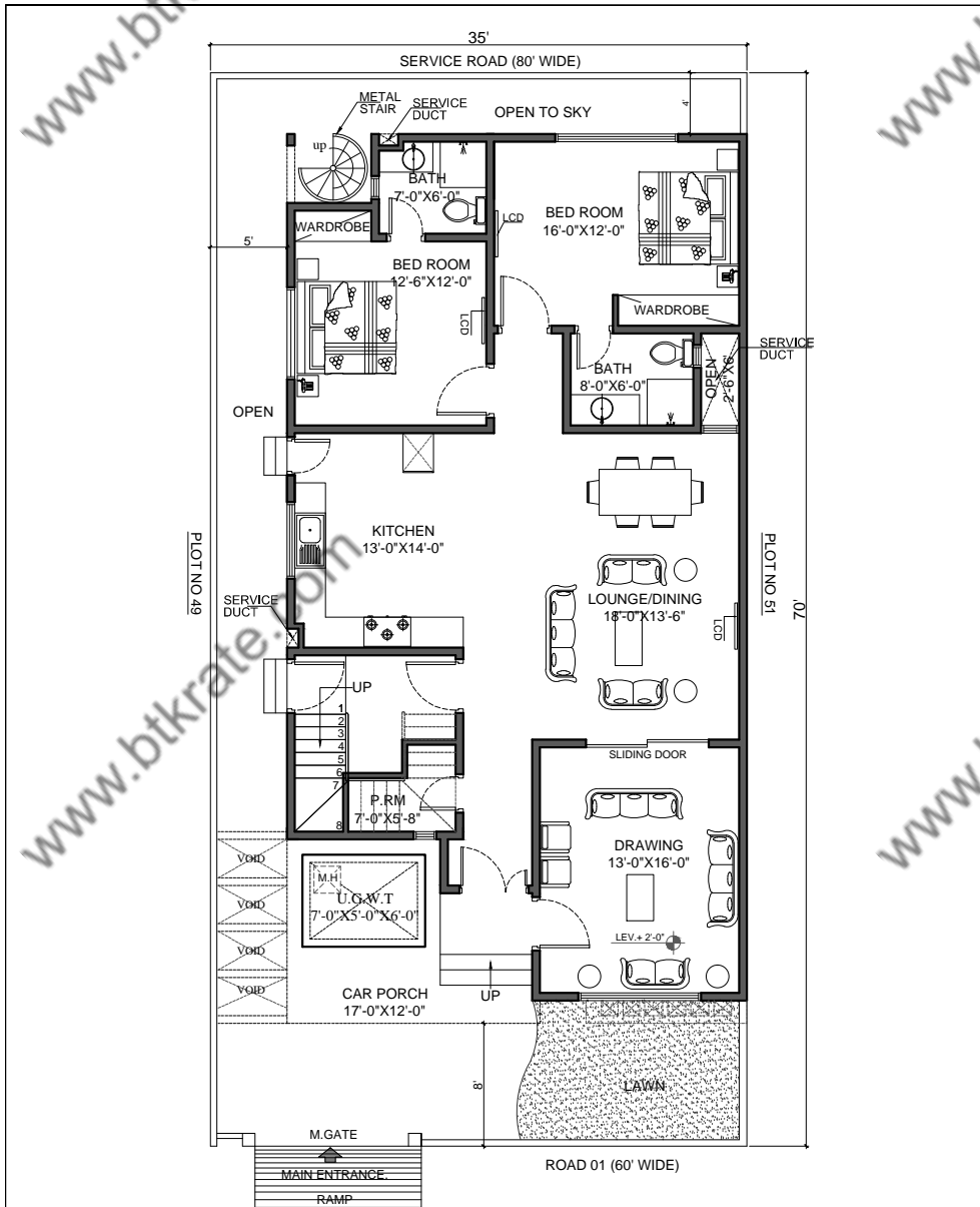
A-01 GROUND FLOOR PLAN
