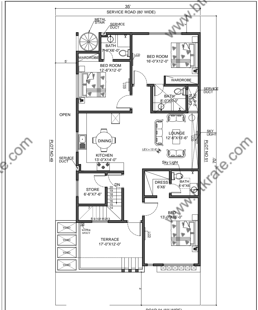
A-02 FIRST FLOOR PLAN
