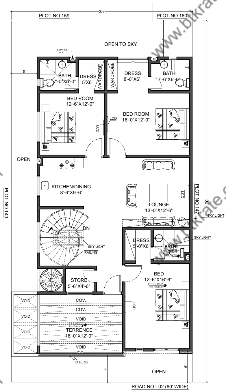
A-02 FIRST FLOOR PLAN
