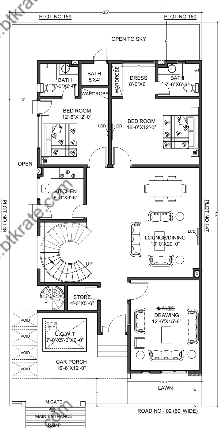
A-01 GROUND FLOOR PLAN
